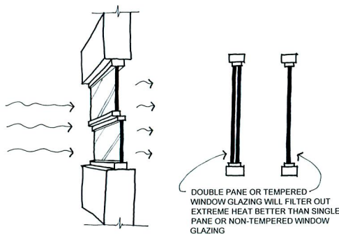
WINDOW GLAZING
