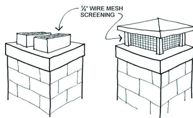
CHIMNEY SCREENS
