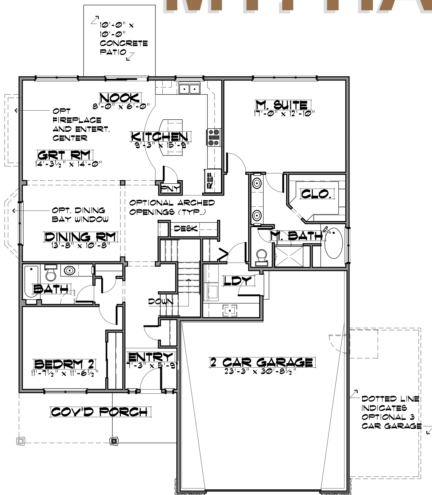
156 - Main Level Floor Plan 1,705 sq. ft.
