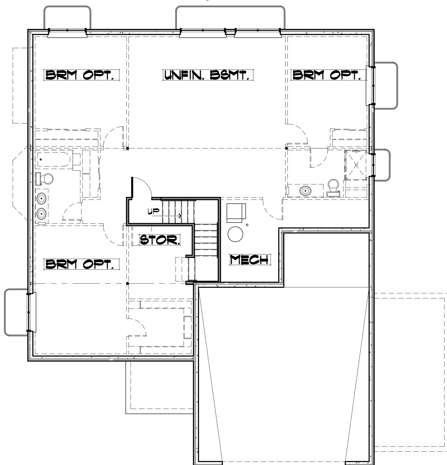
156 - Lower Level Floor Plan 1,500 Unfinished sq. ft.
